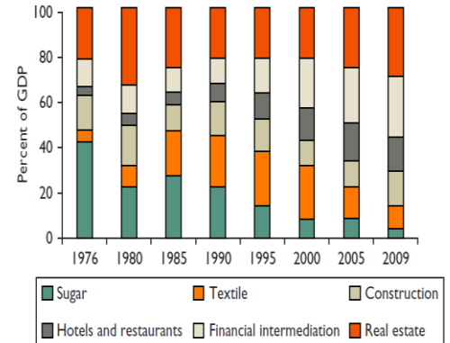
Figure 5.4 Major Economic Sectors in Mauritius, 1976–2009
