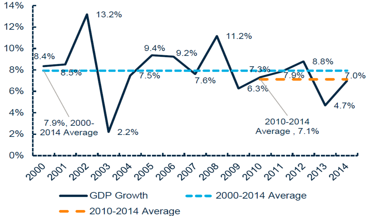
Figure 1.4 Medium and long-term growth
